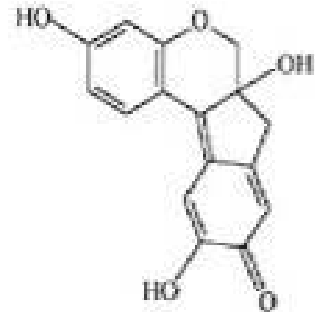
Brazilin
