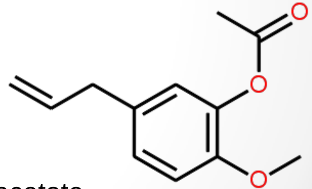
Chavibetol acetate
