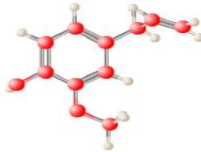
Eugenol ( C_{10}H_{12}O_2 )
