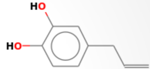
hydroxychavicol
